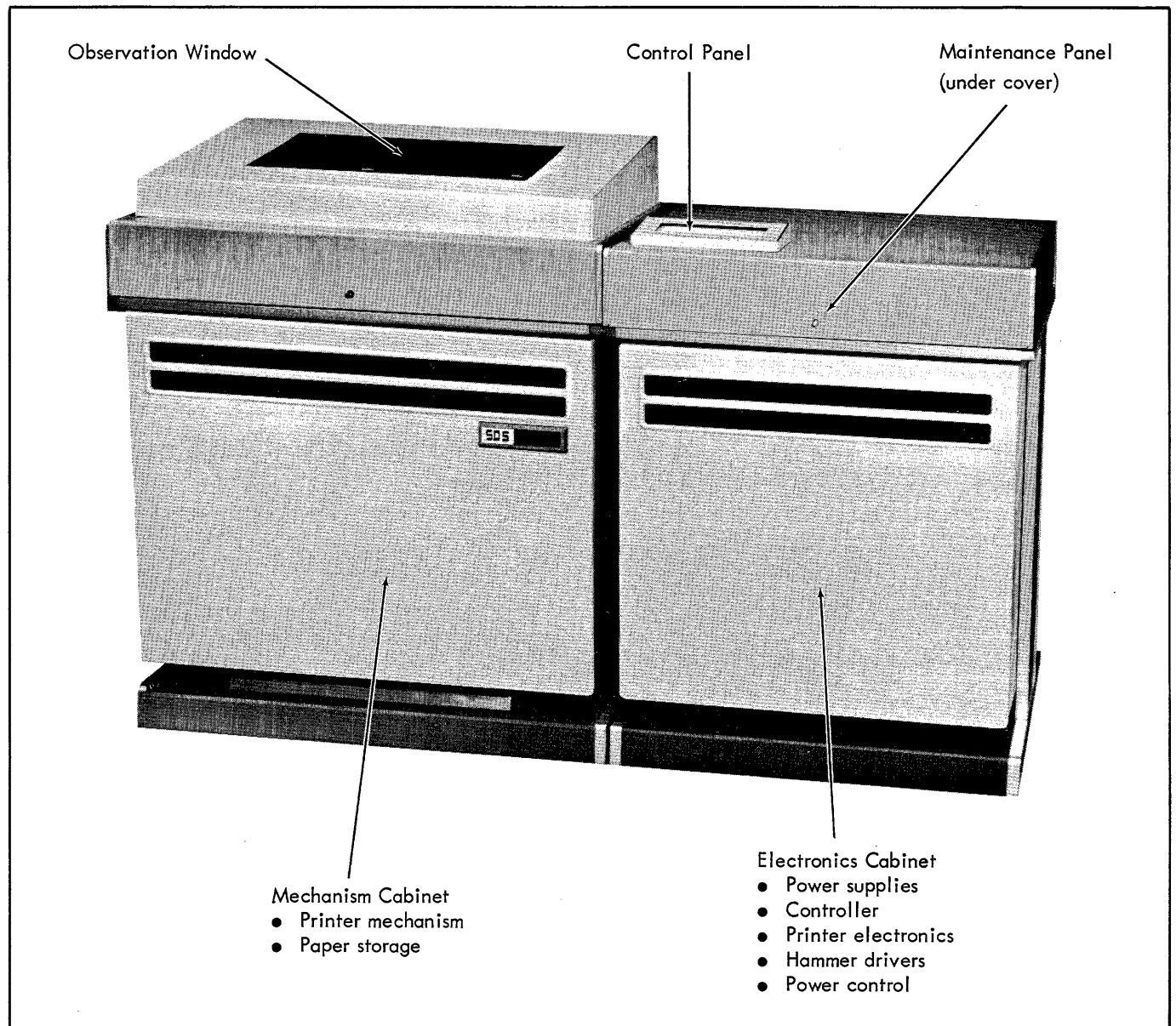
Figure 2. Mechanism and Electronics Cabinets
