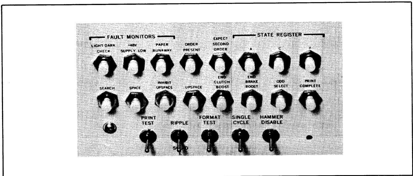
Figure 5. Maintenance Panel
