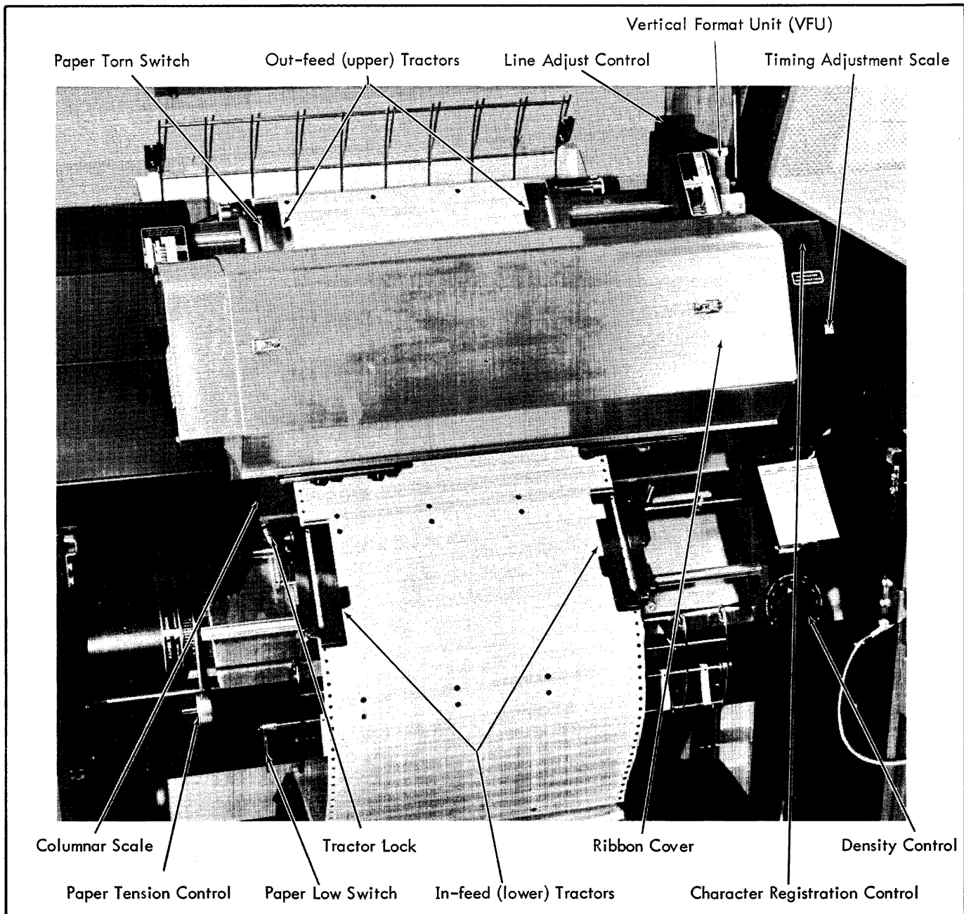
Figure 3. Line Printer Mechanism with Paper Loaded
